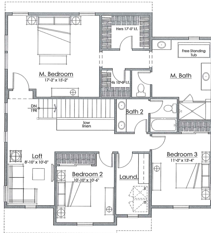
Second Floor 1405 Sq. Ft.
