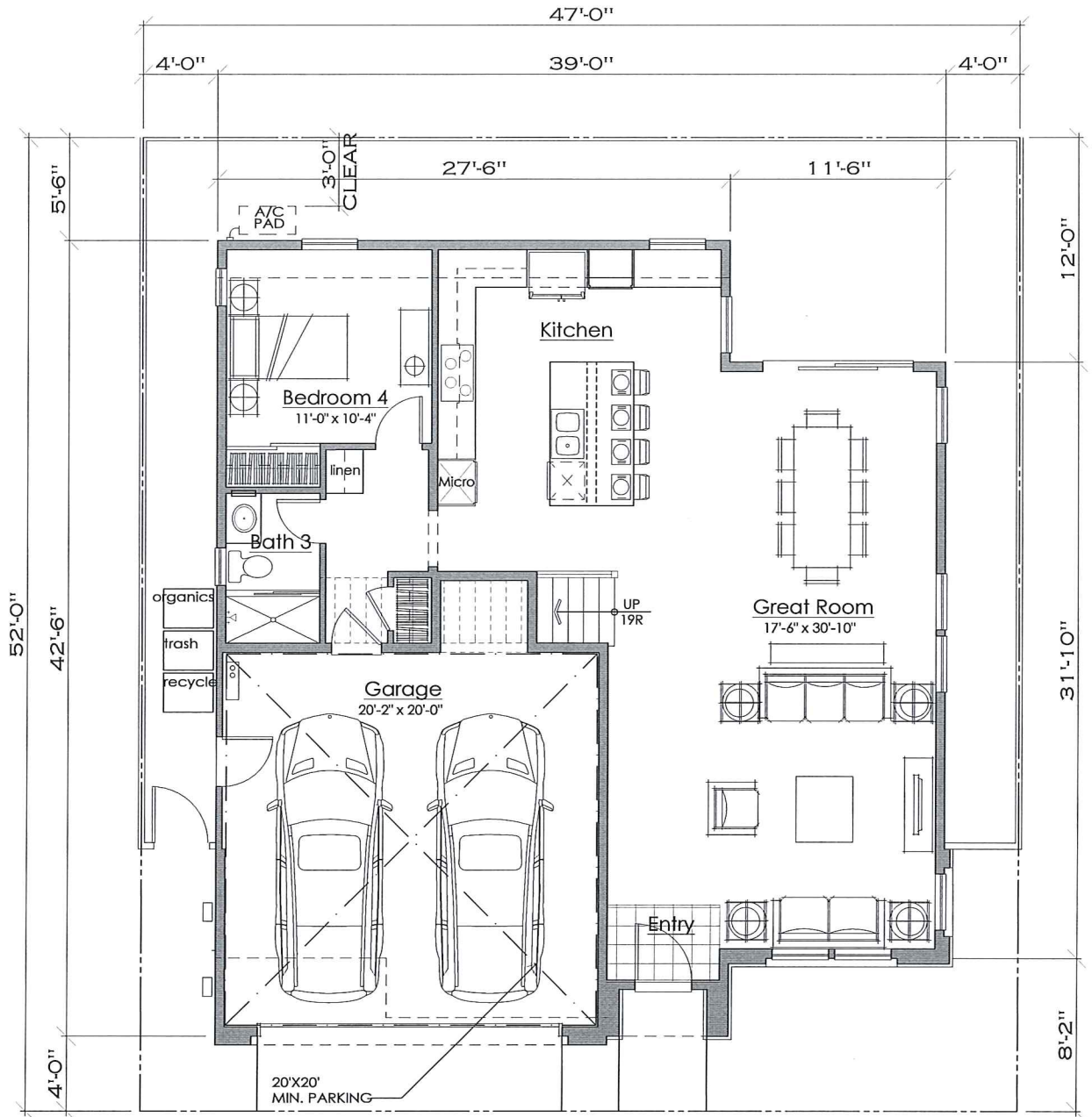
First Floor 1079 Sq. Ft.
