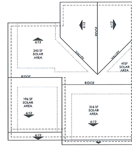
ROOF PLAN OVERHANG: 12" RAKE: 12" ROOF PITCH: 6:12 U.N.O
