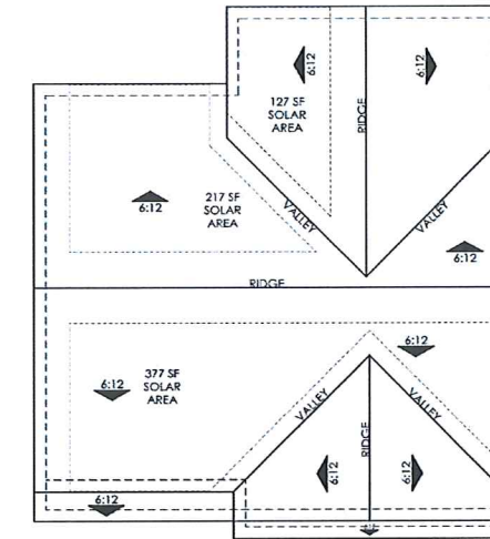
ROOF PLAN OVERHANG: 12" RAKE: 12" ROOF PITCH: 6:12 U.N.O
