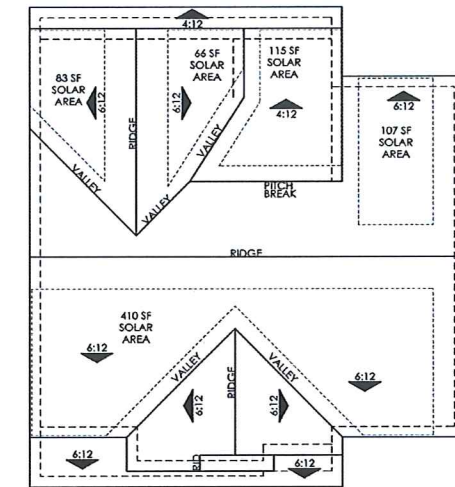
ROOF PLAN OVERHANG: 12" RAKE: 12" ROOF PITCH: 6:12 U.N.O.
