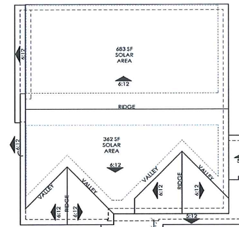
ROOF PLAN OVERHANG: 12" RAKE: 12" ROOF PITCH: 6:12 U.N.O.
