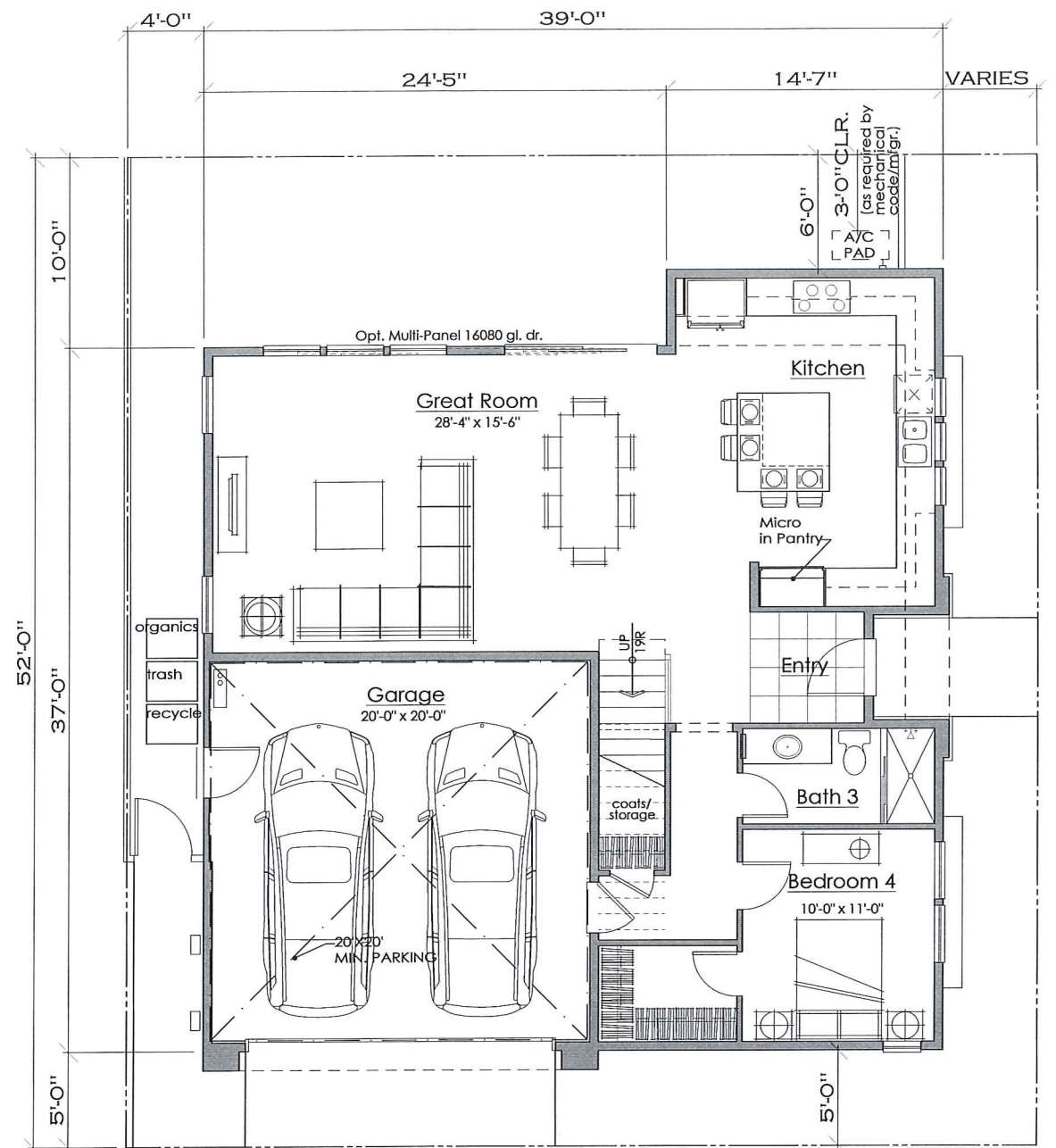
First Floor 1063 Sq. Ft.
