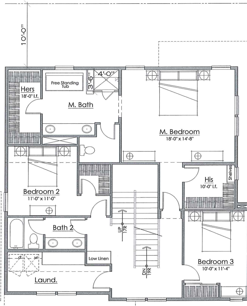
Second Floor 1382 Sq. Ft.
