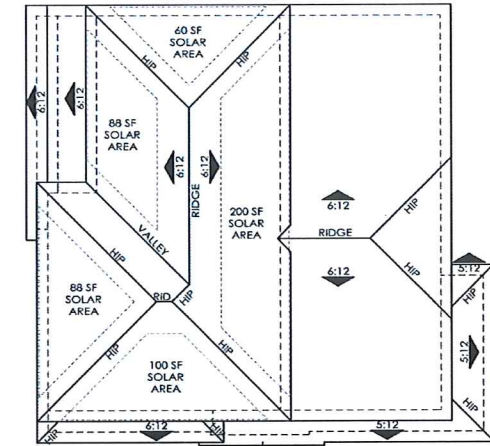
ROOF PLAN OVERHANG: 12" RAKE: 12" ROOF PITCH: 6:12 U.N.O.
