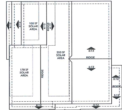
ROOF PLAN OVERHANG: 12" RAKE: 12" ROOF PITCH: 6:12 U.N.O
